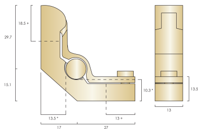
* Distance between Stair Rod fitted with Hinged Fixing Eye and stair tread & riser. + Distance to centre of fixing screw hole.
