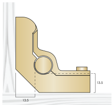
Distance between Stair Rod fitted with Hinged Fixing Eye and stair tread & riser.
