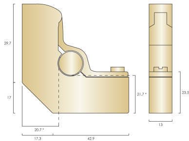
* Distance between Stair Rod fitted with High Style Hinged Fixing Eye and stair tread & riser.
